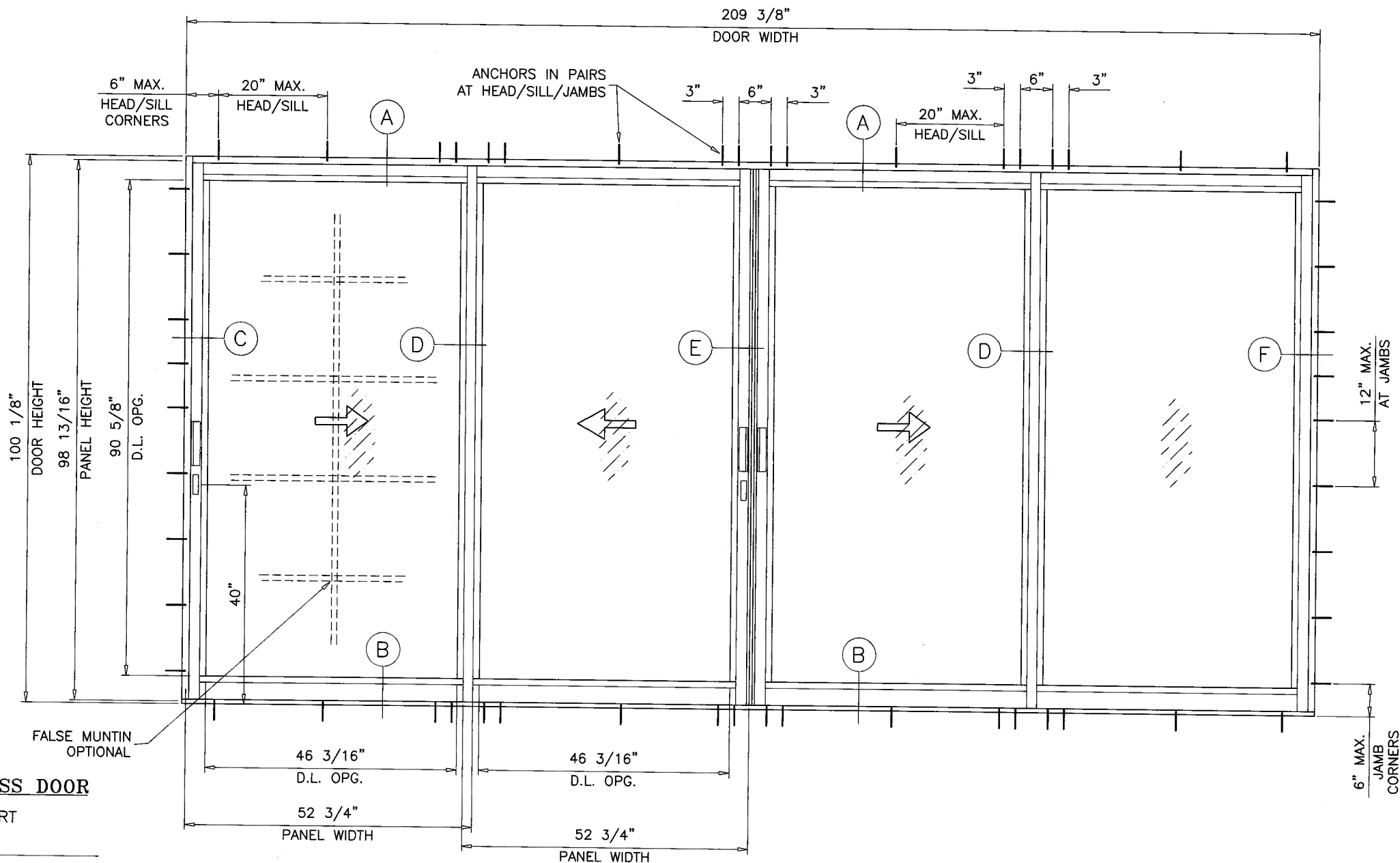
TYPICAL ELEVATION
