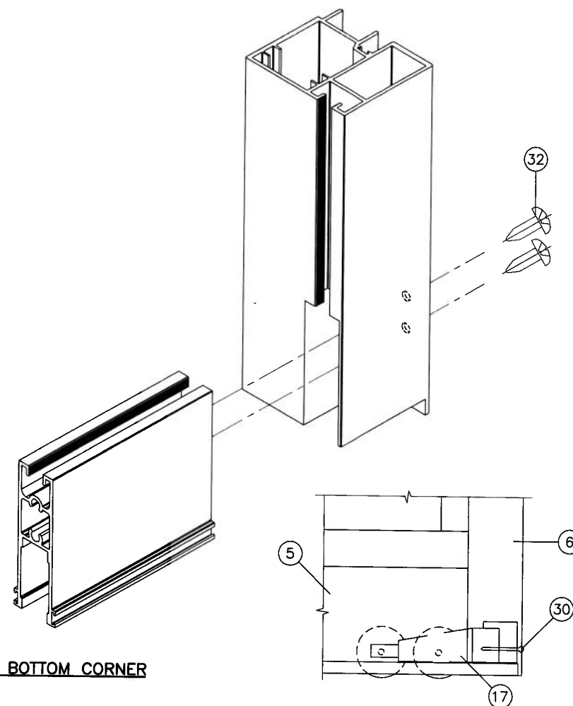
ROLLER FASTENER DETAIL
